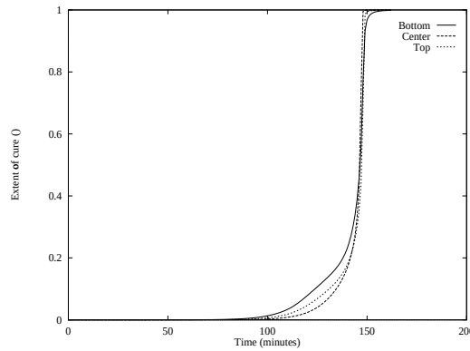
FIG. E.4 – Through thickness curing behaviour
